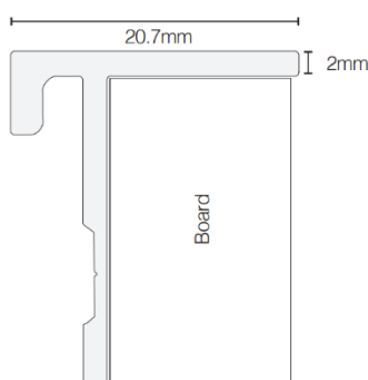
SIDE DETAIL
